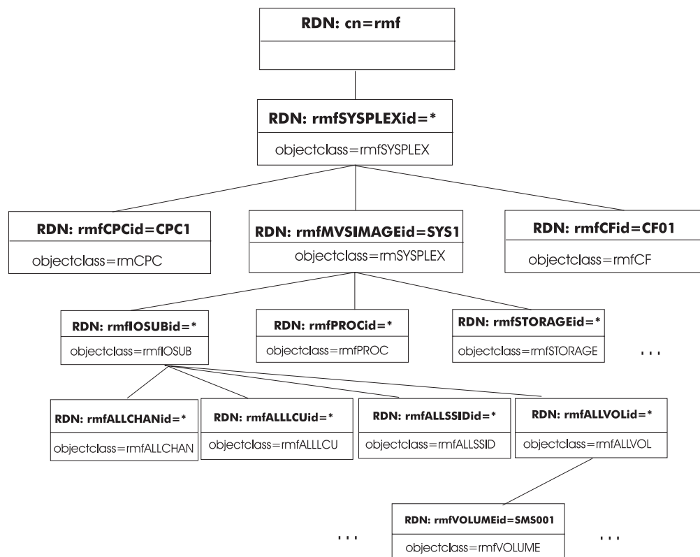
Figure 7. Sample DIT Portion of the RMF LDAP Performance Data
