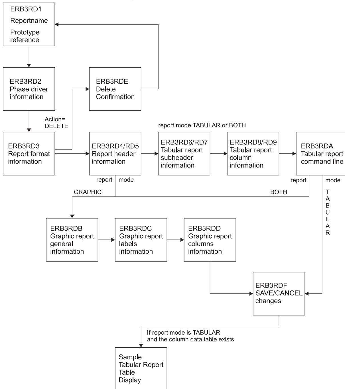
Figure 26. Panel Sequence for the Report Definition Utility
