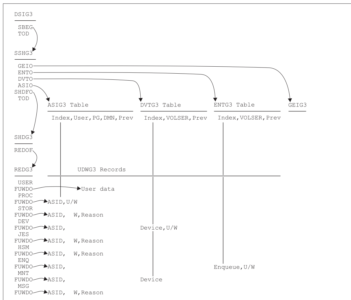
Figure 49. Monitor III Measurement Table and Record Relationships
