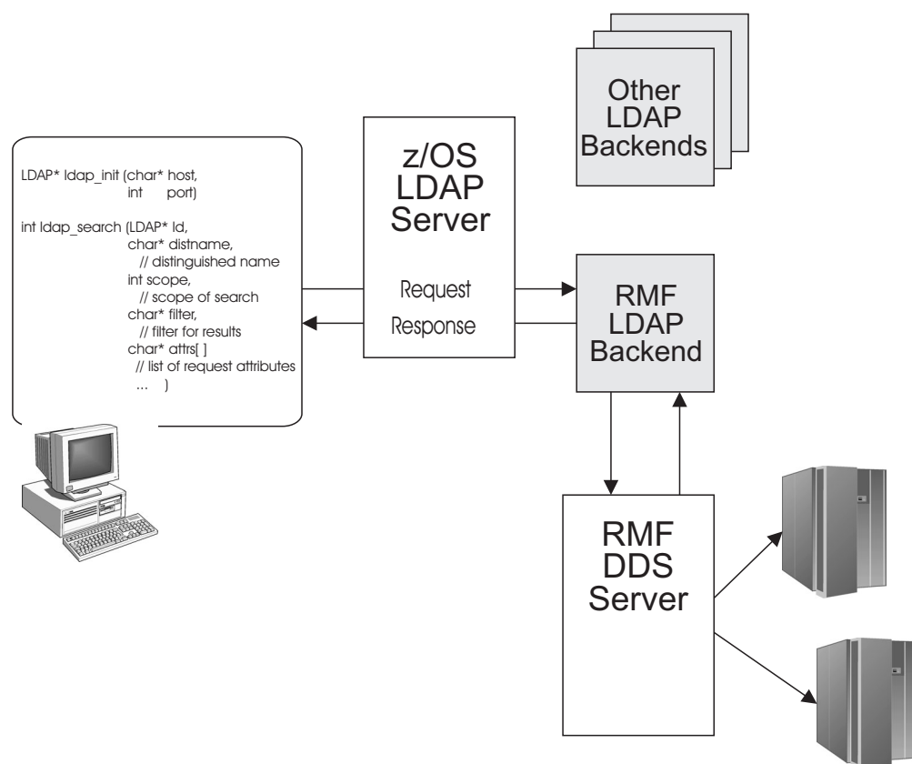
Figure 8. Accessing Performance Data from LDAP
